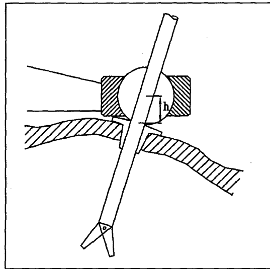
Figure 1: The wrist with spherical joint.
