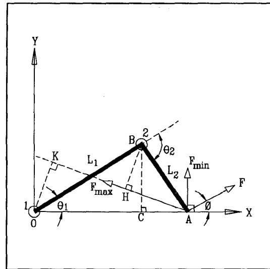
Figure 4: Manipulating forces acting on the arm.
