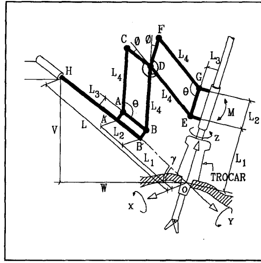
Figure 3: The concentric multi-link spherical joint
