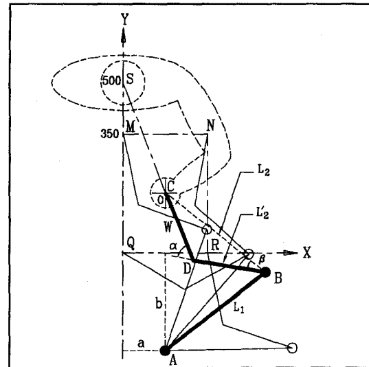
Figure 7: The wrist with orientation toward point S.
