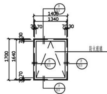
LC1417 防火窗
