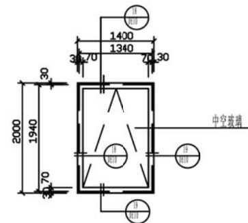
LC1420 合金窗
